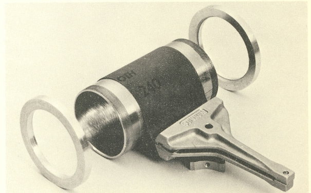
KKN-700 Universal Honing Fixture, HF-300 Workholder, and two loose-fitting End Caps used to fixture Cylinder
