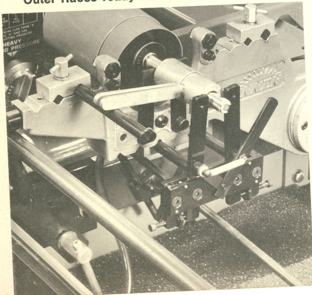
KKN-600 Adjustable Finger Fixture, KKN-720A Fingers, and Customer-Made Pot Fixture used to fixture Outer Races
