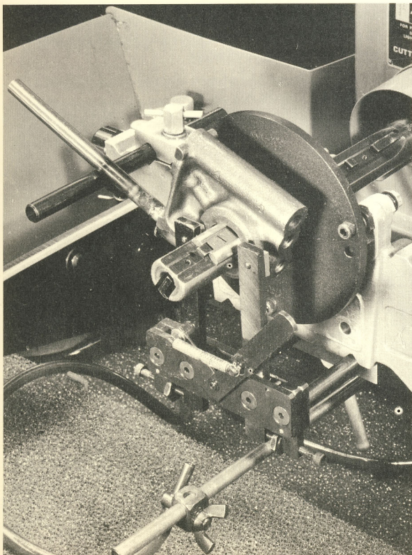
KKN-600 Adjustable Finger Fixture, KKN-209 Face Plate, and Customer-Made Torque Bar used to fixture Bracket
