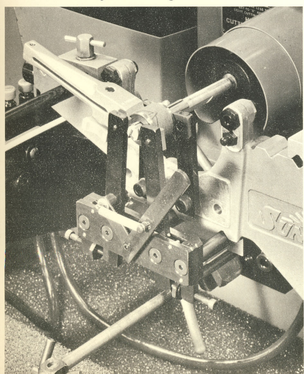
KKN-600 Adjustable Finger Fixture, HF-75 Workholder, and KKN-720A Fingers used to fixture Rollers
