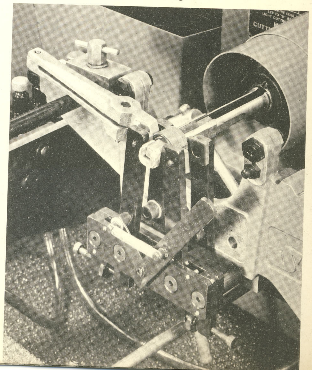
KKN-600 Adjustable Finger Fixture, KKN-720A Fingers, and altered HF-75 Workholder used to fixture Bushing
