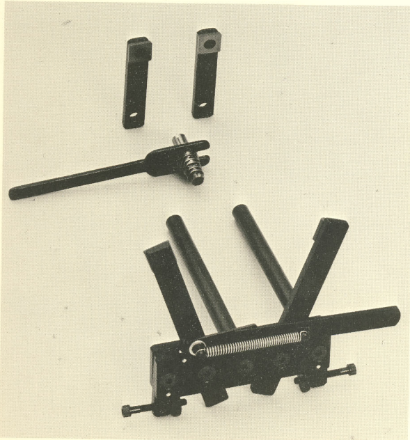
KKN-600 Adjustable Finger Fixture, KKN-720A Fingers, and Customer-Made Torque Absorber which engages flats on the Valve
