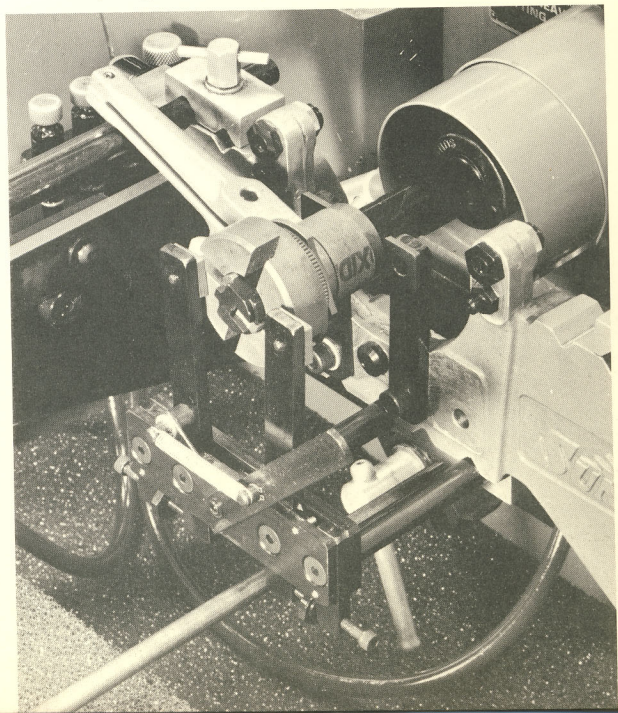
KKN-600 Adjustable Finger Fixture, HF-75 Workholder, and KKN-720A Fingers used to fixture Coupling
