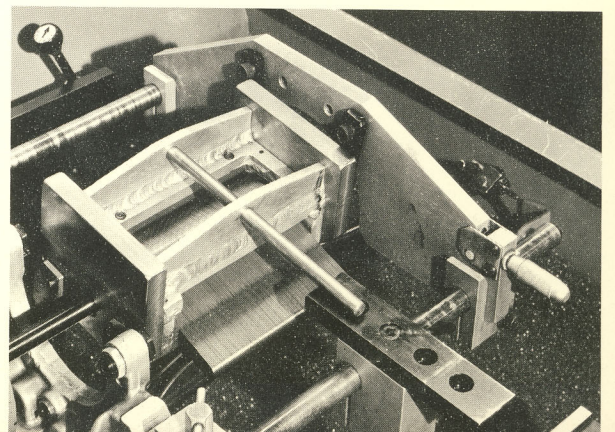
KKN-700 Universal Honing Fixture and Customer-Made Workholder used to fixture Selectors 85 at a time
