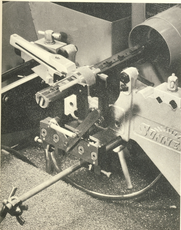
KKN-600 Adjustable Finger Fixture, KKN-720A Fingers, and HF-75 Workholder used to fixture Bushing
