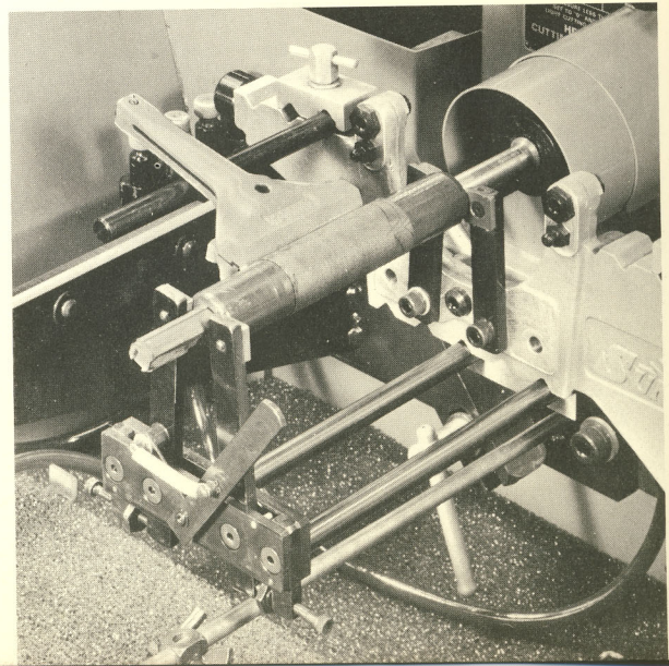
KKN-600 Adjustable Finger Fixture, HF-300 Workholder, and KKN-720A Fingers used to fixture Valve Guide
