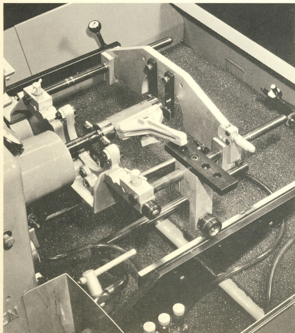
KKN-700 Universal Honing Fixture and HF-300 Workholder used to fixture Wrist Pin
