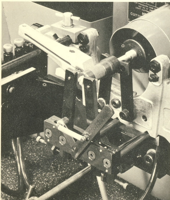
KKN-600 Adjustable Finger Fixture, HF-75 Workholder, and KKN-720A Fingers used to fixture Barrel
