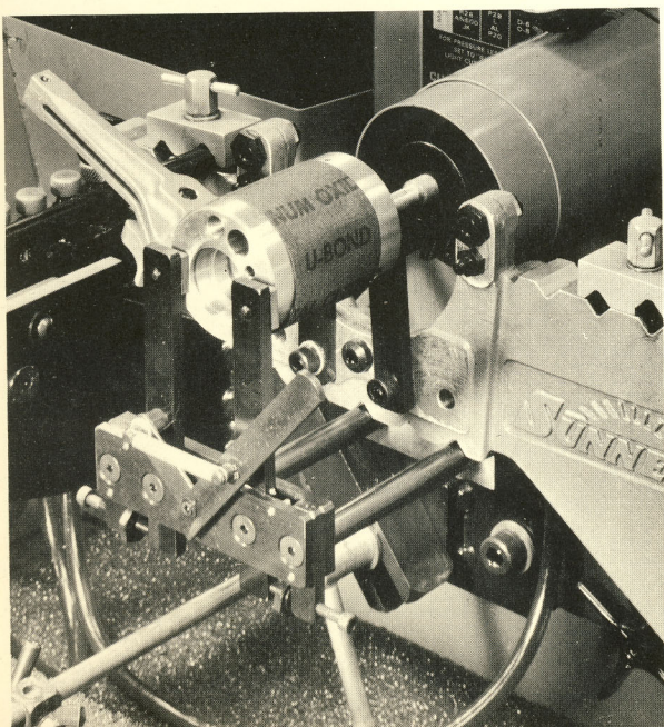
KKN-600 Adjustable Finger Fixture, HF-200 Workholder, and KKN-720A Fingers used to fixture Body
